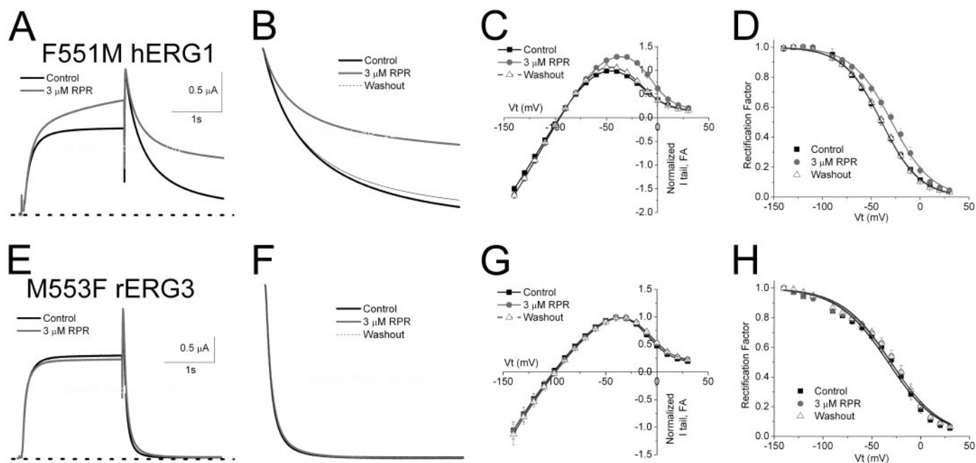
Fig. 3. The variant residue in the S4-S5 linker does not confer differential sensitivity of hERG1 and rERG3 channel currents to RPR. A , effect of 3 \mu M RPR on F551M hERG1 mutant channel currents expressed in an X. laevis oocyte. RPR reversibly enhanced the magnitude and slowed the deactivation rate of F551M hERG1 currents elicited with 2-s pulses to 0 mV from a holding potential of -110 mV. Tail currents were measured at -70 mV. B , RPR significantly slowed F551M hERG1 deactivation. Superimposed tail currents recorded at -70 mV ( n = 5 ) were averaged, normalized relative to their peak value before (Control), during (●), and after washout ( \Delta ) of 3 \mu M RPR. C , fully activated I-V relationships, normalized relative to peak outward current in control, before (control, ■), during (●), and after washout ( \Delta ) of 3 \mu M RPR ( n = 5 ). D , voltage dependence of rERG3 inactivation determined from rectification of the fully activated I-V relationship (same symbols as in C). E-H , 3 \mu M RPR had minimal effect on M553F rERG3 mutant channel currents ( n = 6 ). Protocols and analysis were the same as that described in A-D. Quantitative analysis of the effects of RPR on rates of deactivation and voltage dependence of inactivation of mutant channels are summarized in Tables 1 and 2, respectively.
