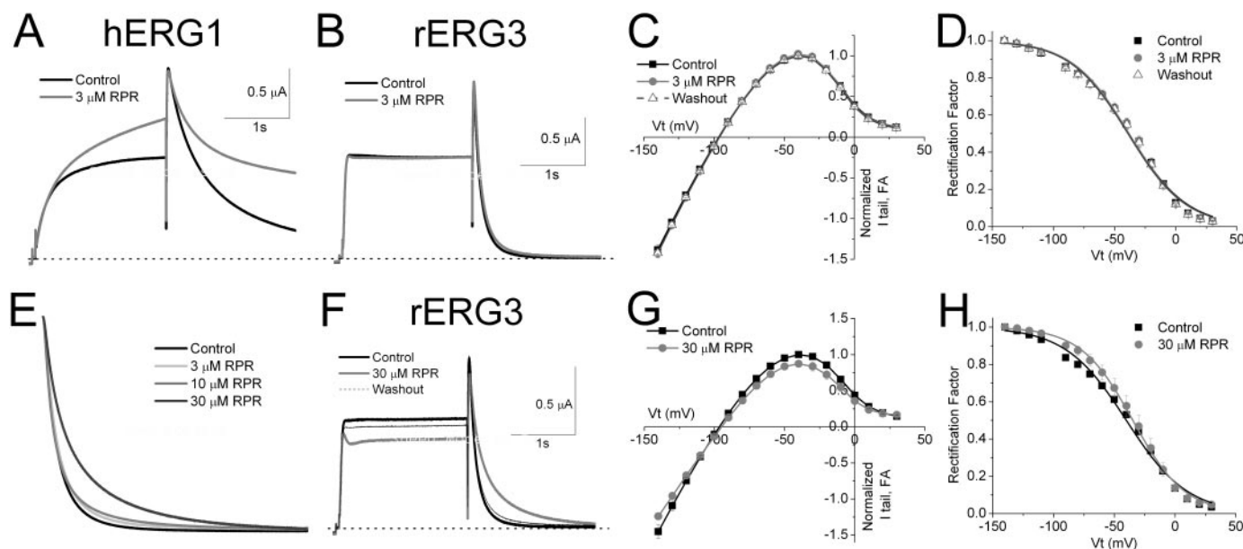
Fig. 1. Comparison of RPR effects on hERG1 and rERG3 channel currents recorded in X. laevis oocytes. A, 3 μM RPR increases the magnitude and slows deactivation of hERG1 current. Currents shown were elicited with 2-s pulses to 0-mV from a holding potential of -110 mV, and tail currents were measured at -70 mV. B to H, effect of RPR on rERG3 channel current. B, at 3 μM, RPR failed to enhance the magnitude of rERG3 channel current and produced only a very small but significant slowing of deactivation. Protocol as in A. C, fully activated I-V relationships, normalized relative to peak outward current in control, before (control, \blacksquare ), during (●), and after washout ( \triangle ) of 3 μM RPR. D, voltage dependence of rERG3 inactivation determined from rectification of the fully activated I-V relationship. Symbols as in C. E, RPR affect on rERG3 deactivation at 3, 10, and 30 μM. Superimposed mean tail currents recorded at -70 mV were normalized relative to their peak value before (Control) and after addition of 3 ( n = 5 ), 10 ( n = 4 ) and 30 μM ( n = 3 ) RPR. F, at 30 μM, RPR produced a partially reversible antagonist effect on rERG3 current. Protocol as in A. G, fully activated I-V relationships, normalized relative to peak outward current in control, before (control, \blacksquare ) and after (●) 30 μM RPR. H, voltage dependence of rERG3 inactivation determined from rectification of the fully activated I-V relationship. Symbols as in G. Thirty micromolar RPR shifted the V_{0.5} by 4.8 \pm 0.3 mV ( n = 3 ) compared with 1.2 \pm 0.7 mV ( n = 3 ) using 0.3% DMSO as control. Quantitative analysis of the effects of RPR on rates of deactivation and voltage-dependence of inactivation of wild-type channels are summarized in Tables 1 and 2, respectively.
