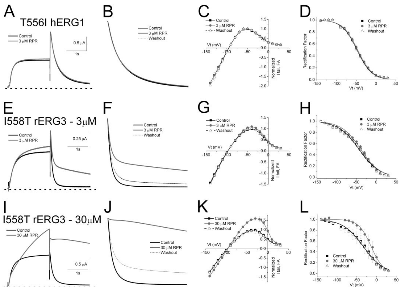
Fig. 4. A variant residue in the S5 domain partially confers differential sensitivity of hERG1 and rERG3 channel currents to RPR. A–D, lack of effect of 3 \mu M RPR on T556I hERG1 mutant channel currents expressed in X. laevis oocytes. A, currents were elicited with 2-s pulses to 0 mV from a holding potential of -110 mV. Tail currents were measured at -70 mV. B, RPR does not slow T556I hERG1 current deactivation. Superimposed tail currents recorded at -70 mV ( n = 5 ) were averaged and then normalized relative to their peak value before (Control), in the presence of 3 \mu M RPR and after washout. C, fully activated I-V relationships, normalized relative to peak outward current in control, before (control, \blacksquare ), during (3 \mu M RPR, \bullet ) and after washout ( \triangle ) of 3 \mu M RPR ( n = 5 ). D, voltage dependence of T556I hERG1 inactivation determined from rectification of the fully activated I-V relationship. E–H, 3 \mu M RPR slows deactivation of I558T rERG3 channels ( n = 7 ). Protocols and analysis were the same as that described in A–D. Quantitative analysis of the effects of RPR on rates of deactivation and voltage dependence of inactivation of mutant channels are summarized in Tables 1 and 2, respectively. I–L, 30 \mu M RPR enhances current magnitude and slows deactivation and activation of I558T rERG3 channels ( n = 3 ). Protocols and analysis were the same as that described in A–D.
