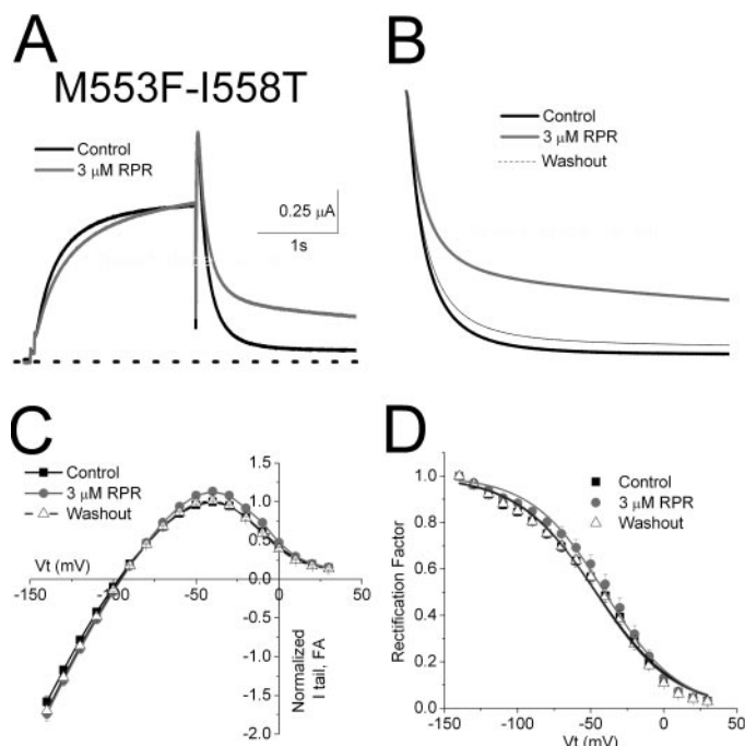
Fig. 5. Effect of 3 \mu M RPR on M553F/I558T rERG3 channel currents. A, currents were elicited with 2-s pulses to 0 mV from a holding potential of -110 mV. Tail currents were measured at -70 mV. B, RPR slows M553F/I558T rERG3 current deactivation. Superimposed tail currents recorded at -70 mV ( n = 4 ) were averaged and then normalized relative to their peak value before (Control), during, and after washout of 3 \mu M RPR. C, fully activated I-V relationships, normalized relative to peak outward current in control ( n = 4 ). D, voltage dependence of inactivation determined from rectification of the fully activated I-V relationship. Quantitative analysis of the effects of RPR on rates of deactivation and voltage dependence of inactivation of M553F/I558T rERG3 channels are summarized in Tables 1 and 2, respectively.
