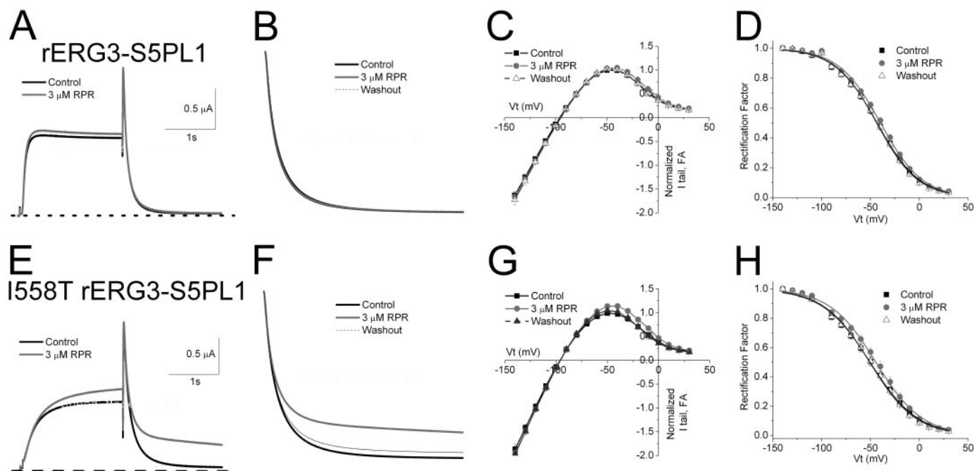
Fig. 6. S5-P linker of ERG channels is not a structural determinant of RPR sensitivity. A–D, effects of 3 \mu M RPR on rERG3-S5PL1 channels (rERG3 with S5-P domain from hERG1). A, currents were elicited with 2-s pulses to 0 mV from a holding potential of -110 mV. B, RPR does not slow rERG3-S5PL1 channel current deactivation. Superimposed tail currents recorded at -70 mV ( n = 6 ) were averaged and then normalized relative to their peak value before (Control), during, and after washout of 3 \mu M RPR. C, fully activated I–V relationships, normalized relative to peak outward current in control, before (control, \blacksquare ), during ( \bullet ), and after washout ( \triangle ) of 3 \mu M RPR ( n = 6 ). D, voltage dependence of inactivation determined from rectification of the fully activated I–V relationship. E–H, 3 \mu M RPR slightly enhances current magnitude and slows deactivation and activation of I558T rERG3-S5PL1 channels ( n = 7 ). Protocols and analysis were the same as that described in A–D. Quantitative analysis of the effects of RPR on rates of deactivation and voltage dependence of inactivation of mutant channels are summarized in Tables 1 and 2, respectively.
